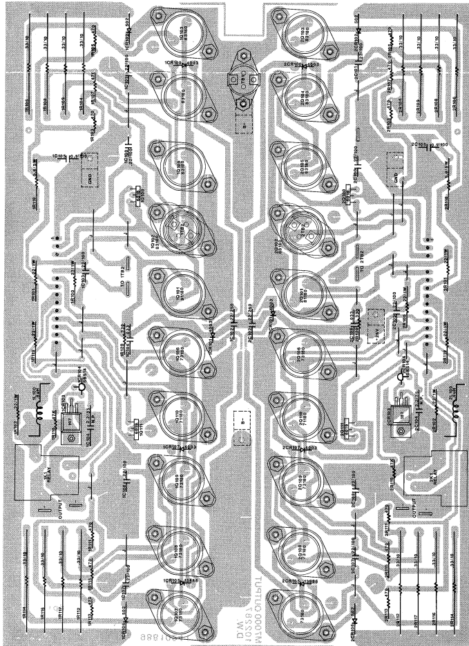
OUTPUT BD.
